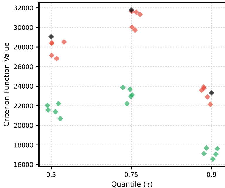
(b) Baseline Volatility (Null Model C_\tau )
