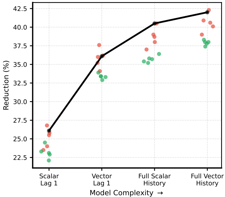
(a) Reduction in Criterion Function ( \tau = 0.9 )
